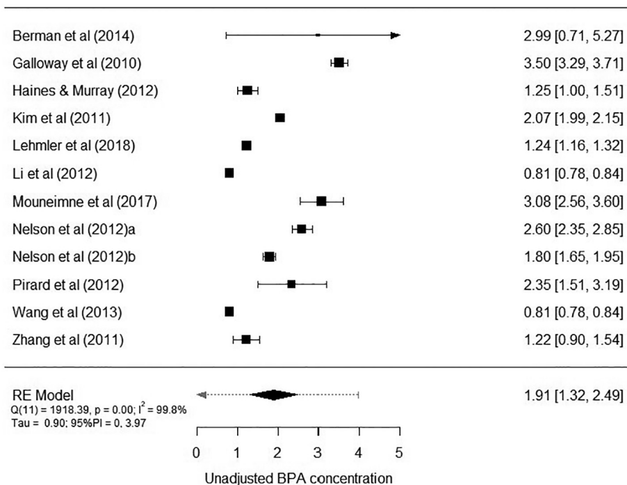
Fig. 2. Forest plot of the median unadjusted urinary BPA concentrations (µg/l) of 12 studies from urine biological samples. 'Nelson et al (a)' and 'Nelson et al (b)' corresponded to the '2003–04' and '2005–06' NHANES samples, respectively. Black squares represent median BPA concentrations extracted from each study, whereas lines represent the 95% confidence limits around them. Black diamond represents the average of the median BPA concentrations. Dotted lines from the black diamond represent the 95% prediction interval limits (95% PI). Tau = between-studies standard deviation ( \tau ). RE model = random-effects model. Data in brackets are the lower and upper 95% confidence limits for the median BPA concentration and for its average.
